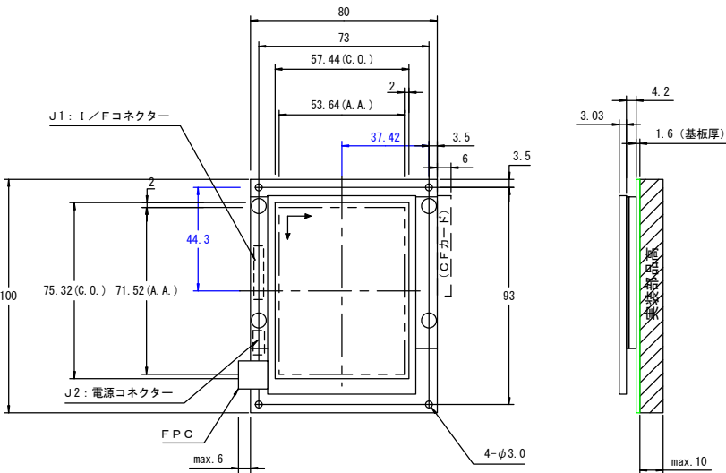
ITC-2432-035C (240×320dot)
